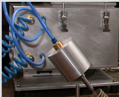
NDF100-3FI on platform balance (top) with additional container (left) with new digital pressure controllers (right)
